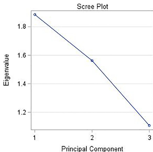
Fig. 2. Scree Plot of Eigenvalues.
