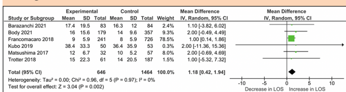
Figure 5. The mean length of LOS in the sarcopenia and non-sarcopenia cohorts
